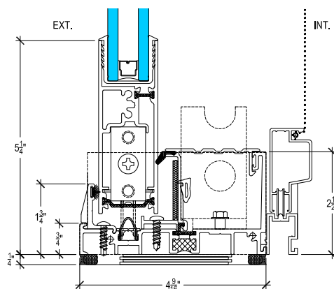
SILL
