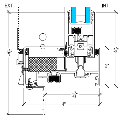
SILL
