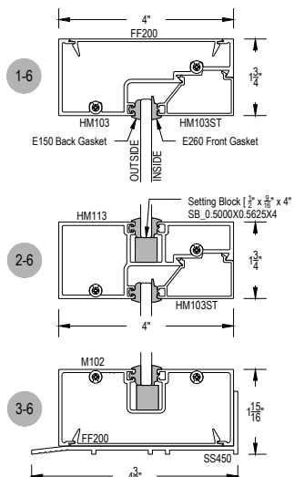
SCREW SPLINE INSIDE SET
