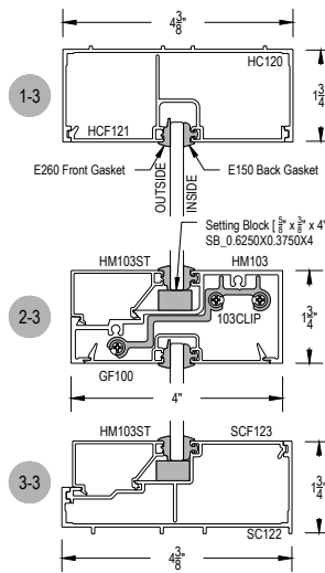
COMPENSATING STICK OUTSIDE SET
