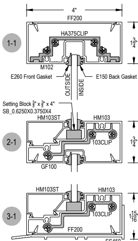
SHEAR BLOCK OUTSIDE SET
