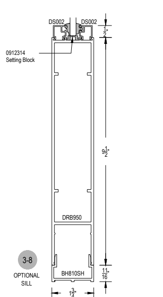
SCREW SPLINE OUTSIDE SET
