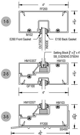
SCREW SPLINE OUTSIDE SET
