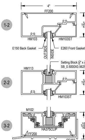
SHEAR BLOCK INSIDE SET
