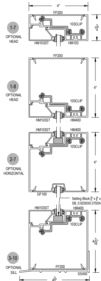
GASKET PLACEMENT FOR INSIDE/OUTSIDE SET SYSTEMS
