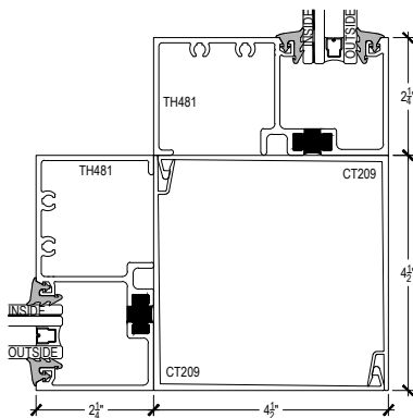
6-1 90° CORNER ASSEMBLY
