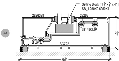
SHEAR BLOCK OUTSIDE SET
