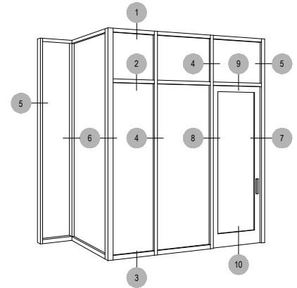
GASKET PLACEMENT FOR 1 3/8" POCKET
