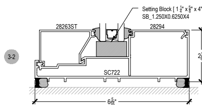
COMPENSATING STICK OUTSIDE SET
