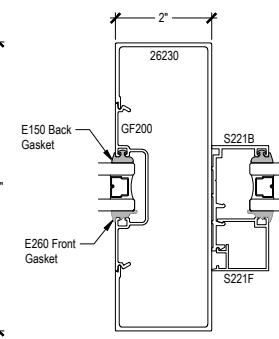
VERTICAL @ TRANSOM
