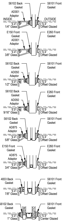
GASKET PLACEMENT FOR 1 3/8" POCKET
