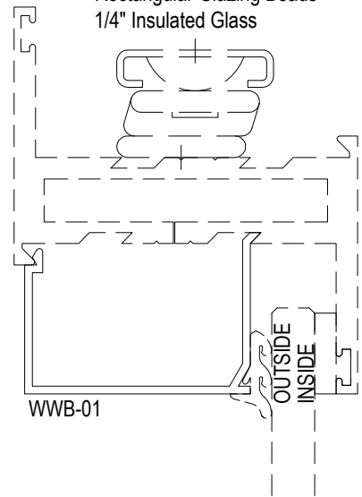
Rectangular Glazing Beads 1/4" Insulated Glass
