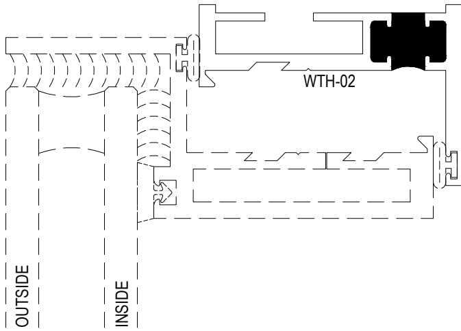
INSULATED GLASS SASH
