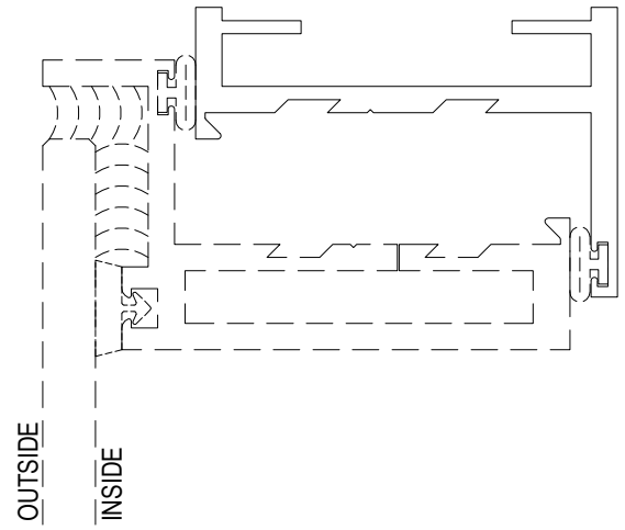
MONOLITHIC GLASS SASH
