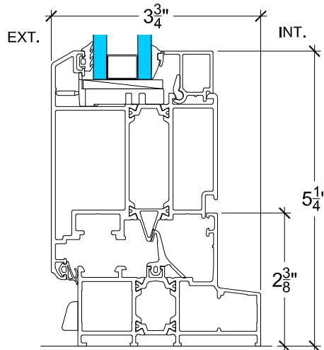
2 3/8" SILL
