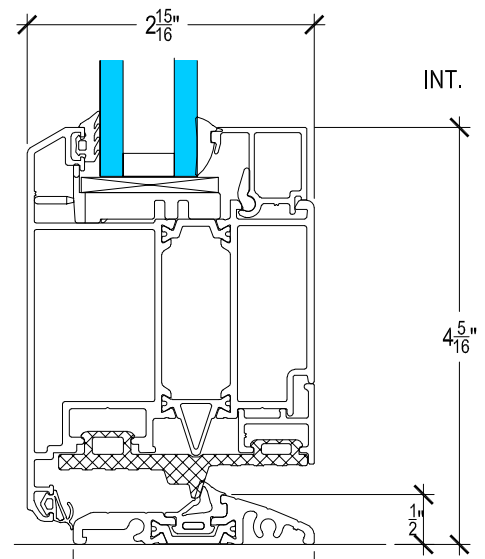
FLUSH SILL
