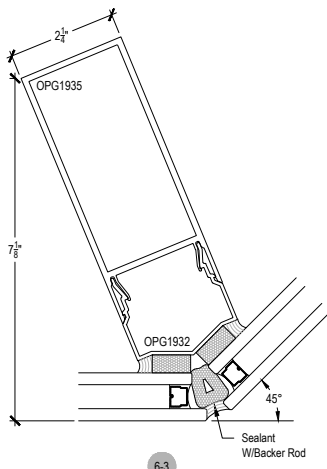
6-3 135° CORNER ASSEMBLY
