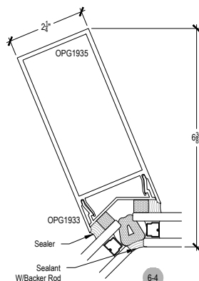
6-4 135° CORNER ASSEMBLY
