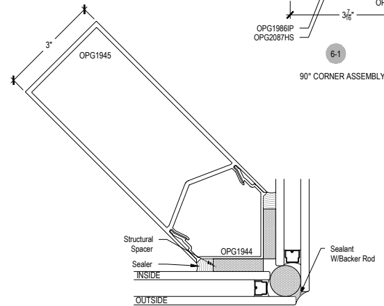
6-2 90° CORNER ASSEMBLY
