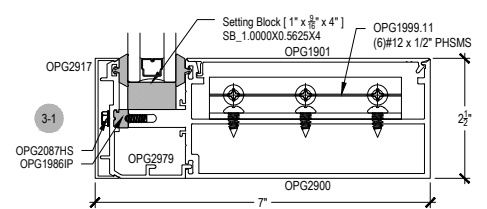
SHEAR BLOCK INSIDE SET
