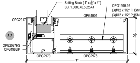
SHEAR BLOCK OUTSIDE SET
