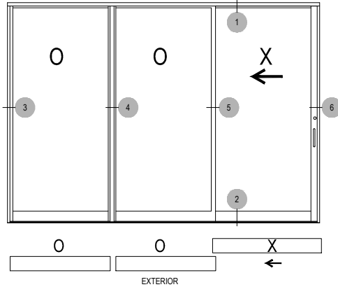
OOX CONFIGURATION EXTERIOR ELEVATION (INSIDE SLIDER SHOWN OUTSIDE SLIDER-AVAILABLE)
