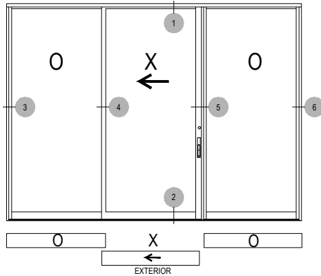
OXRO CONFIGURATION EXTERIOR ELEVATION (OUTSIDE SLIDER SHOWN INSIDE SLIDER-AVAILABLE)
