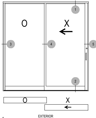
OX CONFIGURATION EXTERIOR ELEVATION (OUTSIDE SLIDER SHOWN INSIDE SLIDER-AVAILABLE) (INTERIOR SCREEN)
