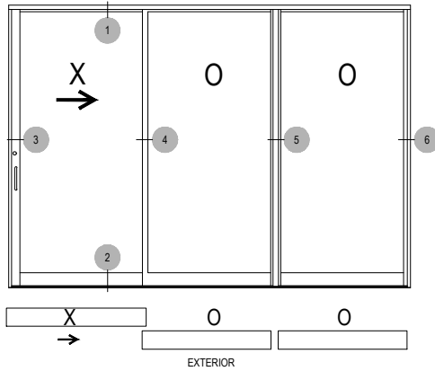
XOO CONFIGURATION EXTERIOR ELEVATION (INSIDE SLIDER SHOWN OUTSIDE SLIDER-AVAILABLE)
