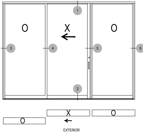
OXRO CONFIGURATION EXTERIOR ELEVATION (INSIDE SLIDER SHOWN OUTSIDE SLIDER-AVAILABLE)
