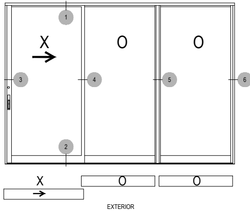
XOO CONFIGURATION EXTERIOR ELEVATION (OUTSIDE SLIDER SHOWN INSIDE SLIDER-AVAILABLE)
