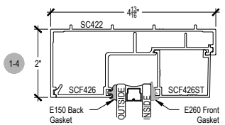
SHEAR BLOCK OUTSIDE SET
