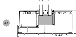
COMPENSATING STICK OUTSIDE SET
