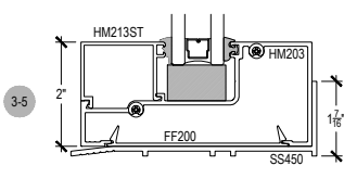
SCREW SPLINE OUTSIDE SET
