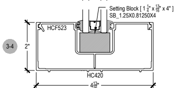
COMPENSATING STICK INSIDE SET
