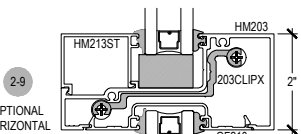
SCREW SPLINE OUTSIDE SET
