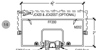
SHEAR BLOCK INSIDE SET
