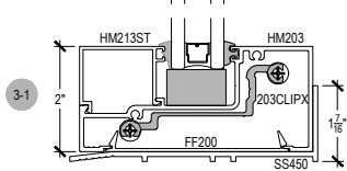
SHEAR BLOCK OUTSIDE SET
