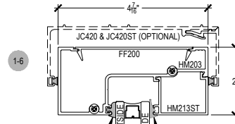
COMPENSATING STICK OUTSIDE SET
