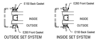
OUTSIDE SET SYSTEM INSIDE SET SYSTEM
