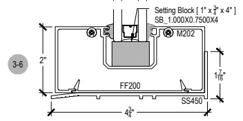
SCREW SPLINE INSIDE SET
