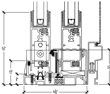
2 2 1/2" B/L SILL
