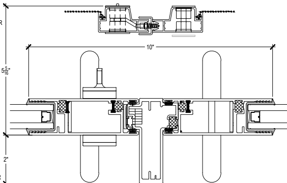
5 MEETING STILES
