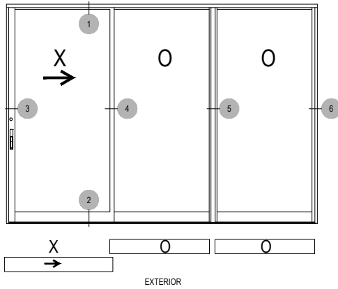
XOO CONFIGURATION EXTERIOR ELEVATION OUTSIDE SLIDER
