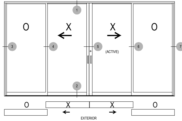
OXXO CONFIGURATION EXTERIOR ELEVATION OUTSIDE SLIDER
