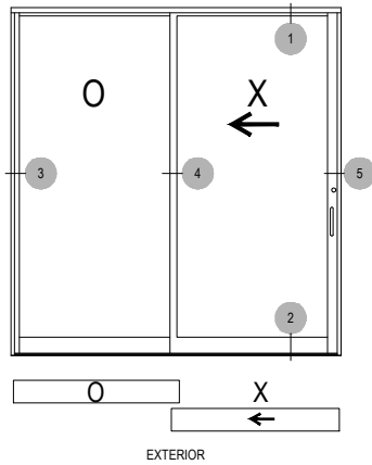
OX CONFIGURATION EXTERIOR ELEVATION OUTSIDE SLIDER (INTERIOR SCREEN)
