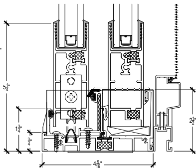
2 2 1/2" B/L SILL
