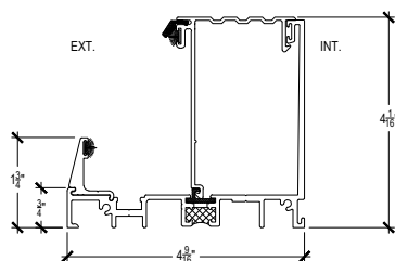
4" B/L SILL
