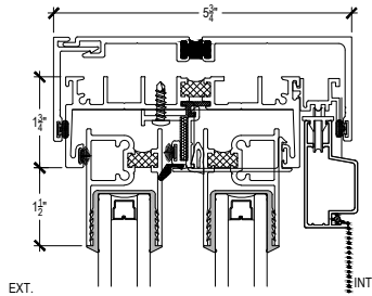
HEAD with 2 Pc HEAD COMP
