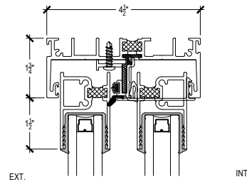
4 1/2" HEAD
