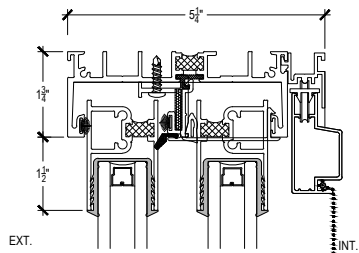
1 HEAD
