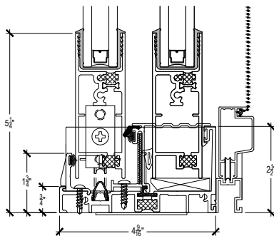
2 2 1/2" B/L SILL
