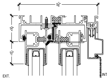
1 HEAD
