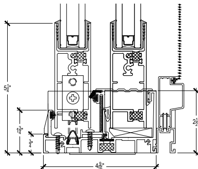
2 2 1/2" B/L SILL
