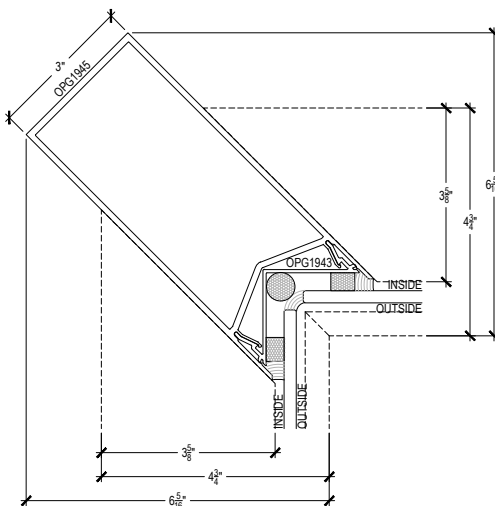
90° SSG INSIDE CORNER
