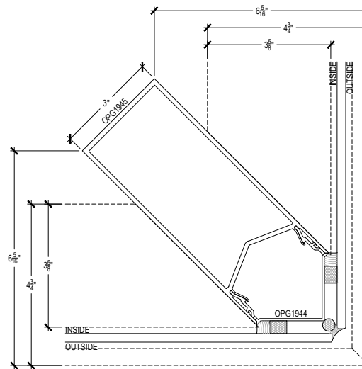
90° SSG OUTSIDE CORNER
