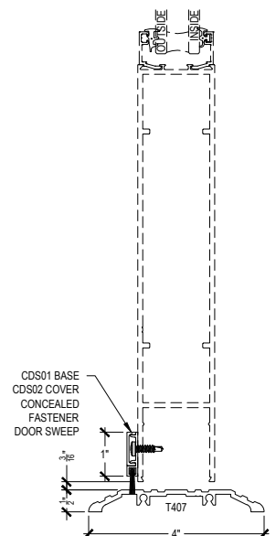
OPTIONAL THRESHOLDS @ CENTER HUNG DOOR
