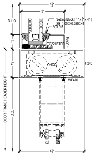
DOOR HEADER CONCEALED CLOSER
