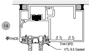
Offset Glazed
