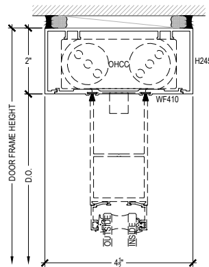
DOOR HEADER CONCEALED CLOSER @ PUNCHED OPENING
