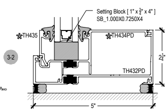
COMPENSATING STICK OUTSIDE SET
