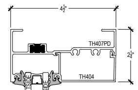
HEAD @ TRANSOM PUNCHED
