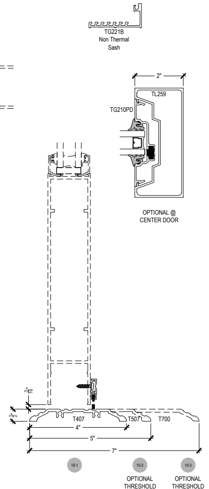
9-4 OPTIONAL VERTICAL @ CENTER DOOR
