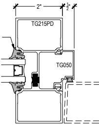
8-2 OPTIONAL VERTICAL @ OFFSET DOOR
