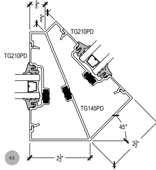
135° CORNER ASSEMBLY
