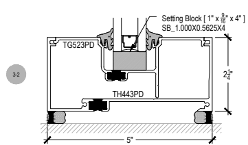
COMPENSATING STICK INSIDE SET
