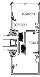
8-3 VERTICAL @ CENTER DOOR
