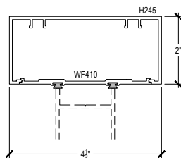
11-3 HEAD @ PUNCHED CENTER DOOR
