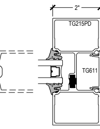
8-4 OPTIONAL VERTICAL @ CENTER DOOR
