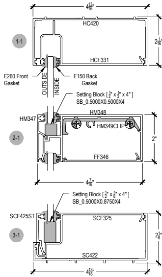
COMPENSATING STICK OUTSIDE SET
