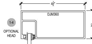
COMPENSATING STICK INSIDE SET
