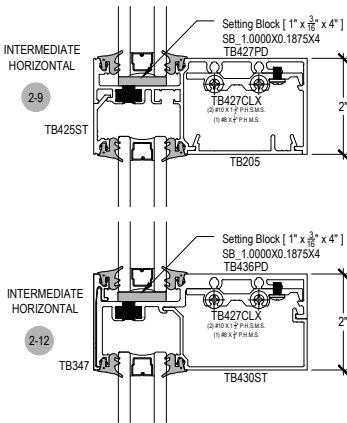
Offset Glazed
