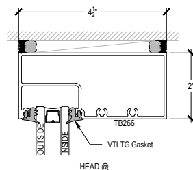
HEAD @ PUNCHED TRANSOM
