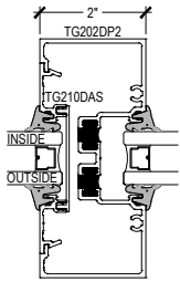
INTERMEDIATE VERTICAL
