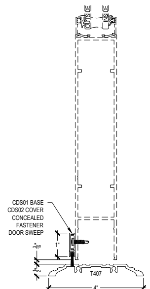
OPTIONAL THRESHOLDS @ CENTER HUNG DOOR
