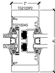
OPTIONAL HEAVY WALL INTERMEDIATE VERTICAL
