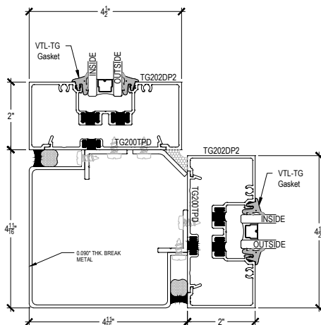
90° CORNER ASSEMBLY
