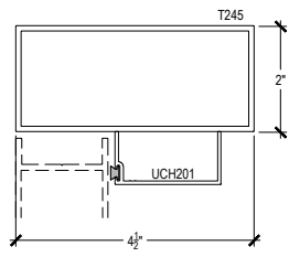
11-2 HEAD @ PUNCHED OFFSET DOOR
