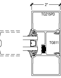
8-4 OPTIONAL VERTICAL @ CENTER DOOR
