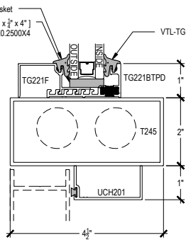
9-2 HORIZONTAL @ OFFSET DOOR W/ CONCEALED CLOSURE
