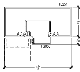
11-1 HEAD @ PUNCHED OFFSET DOOR
