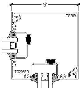
90° CORNER ASSEMBLY
