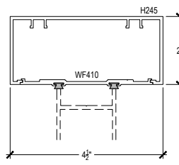
11-3 HEAD @ PUNCHED CENTER DOOR
