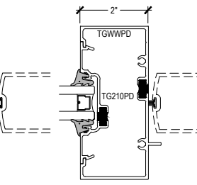
8-5 OPTIONAL VERTICAL @ CENTER DOOR
