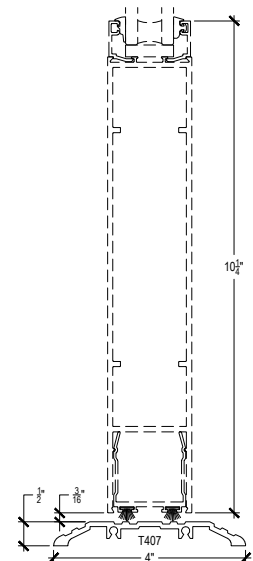
THRESHOLD @ CENTER DOOR
