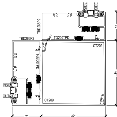
90° CORNER ASSEMBLY
