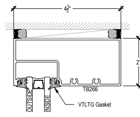
HEAD @ PUNCHED TRANSOM
