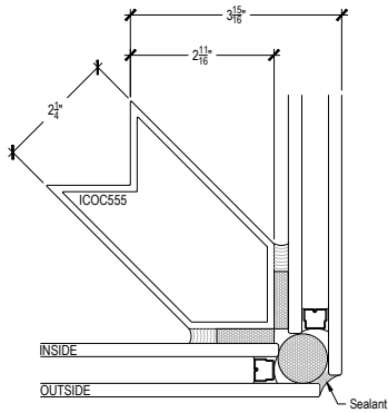
90° OUTSIDE CORNER
