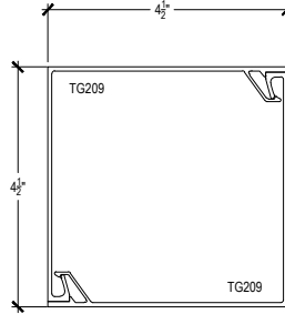
4 1/2 TUBE ASSEMBLY
