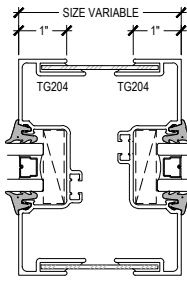
VARIABLE VERTICAL ASSEMBLY
