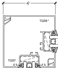
90° CORNER SCREW RACE ASSEMBLY
