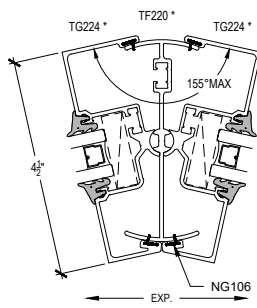
180-155° FLEXIBLE CORNER ASSEMBLY
