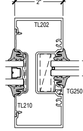
INTERMEDIATE VERTICAL w/ADAPTOR AND GLASS OPTION
