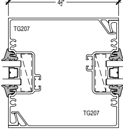
4 1/2" VERTICAL ASSEMBLY
