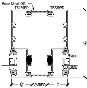
EXPANSION INTERMEDIATE VERTICAL
