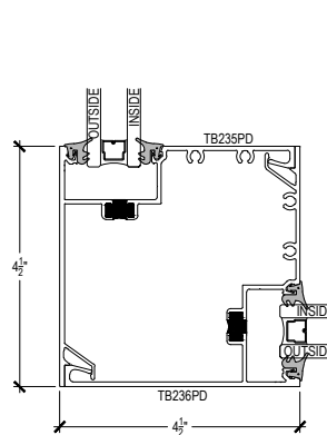
90° CORNER ASSEMBLY 6-4
