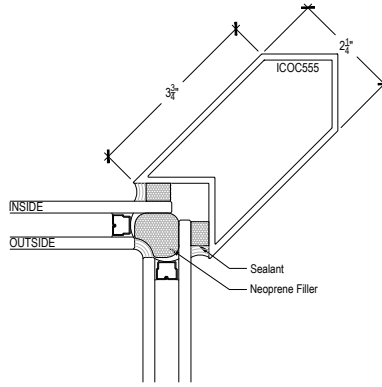
90° INSIDE CORNER 6-2
