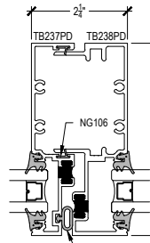
MALE/FEMALE EXPANSION INTERMEDIATE VERTICAL
