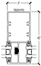
INTERMEDIATE VERTICAL
