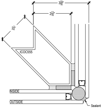
90° OUTSIDE CORNER 6-1
