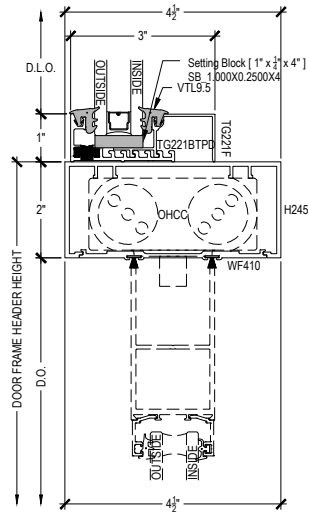
DOOR HEADER CONCEALED CLOSER 9-3
