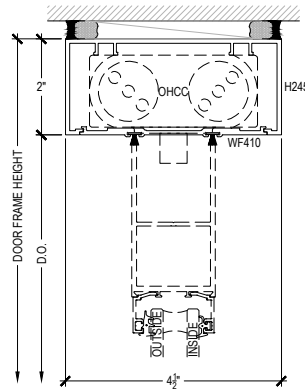
DOOR HEADER CONCEALED CLOSER @ PUNCHED OPENING 11-3
