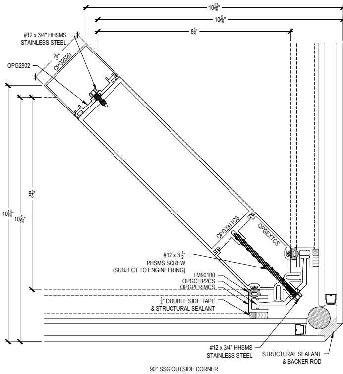
90° SSG OUTSIDE CORNER
