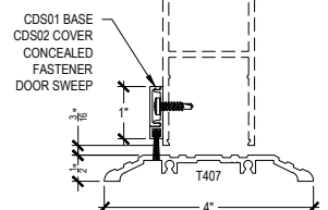
OPTIONAL THRESHOLDS @ CENTER HUNG DOOR
