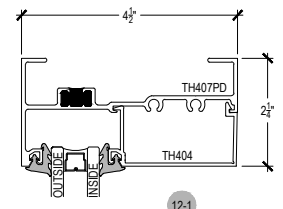
HEAD @ TRANSOM PUNCHED
