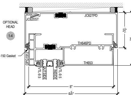
SHEAR BLOCK INSIDE SET Continuous Head / Sill
