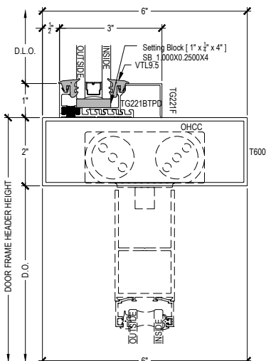
DOOR HEADER CONCEALED CLOSER
