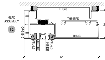
Offset Glazed
