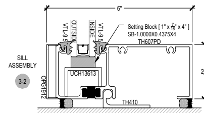
SHEAR BLOCK INSIDE SET Continuous Head / Sill
