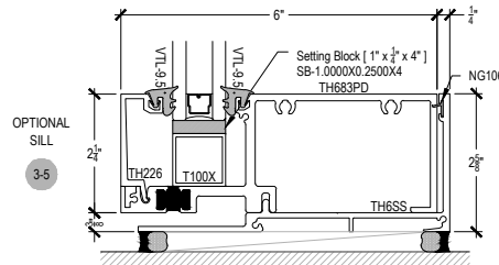
Offset Glazed
