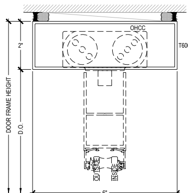
DOOR HEADER CONCEALED CLOSER @ PUNCHED OPENING
