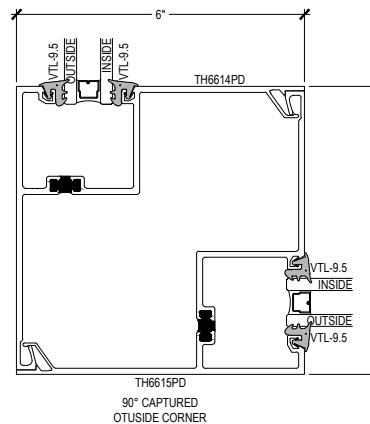
90° CAPTURED OUTSIDE CORNER
