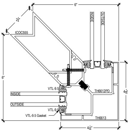
90° CAPTURED OUTSIDE CORNER
