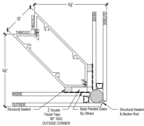
90° SSG OUTSIDE CORNER
