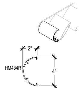
1-8 Open 4" Bullnose
