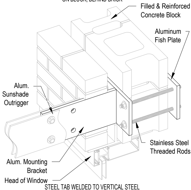
STEEL TAB WELDED TO VERTICAL STEEL
