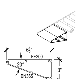
1-16 Closed Deep Angular
