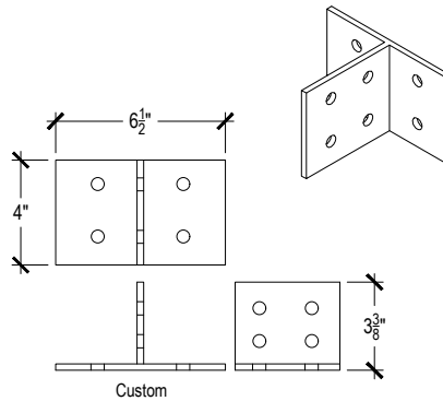
3-5 "T" Bracket
