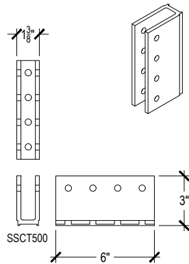
3-1 Square Bracket
