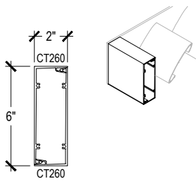
1-5 Closed 6" Rectangular
