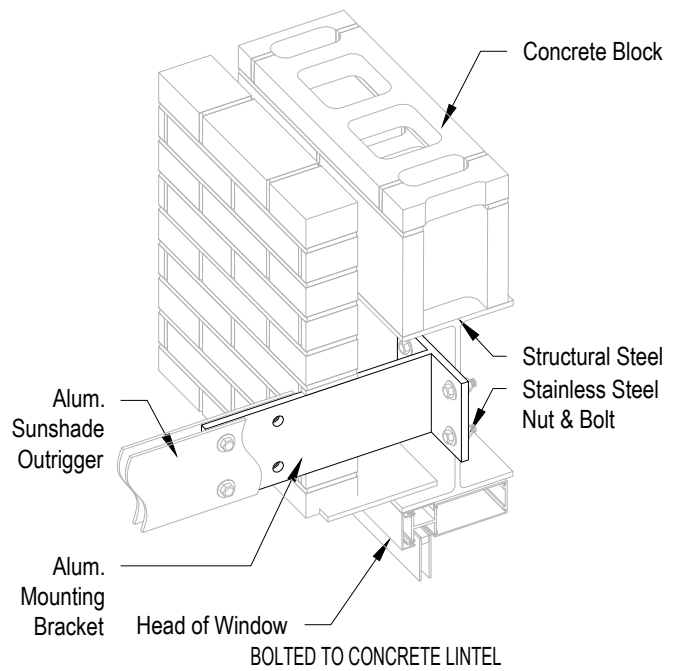
BOLTED TO STEEL BEHIND BRICK
