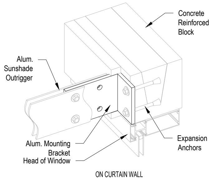
ON CURTAIN WALL
