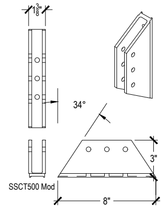
3-3 Tapered Bracket
