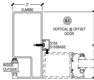
Offset Glazed
