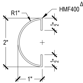
Offset Glazed
