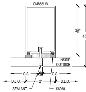
SSG VERTICAL 4-2
