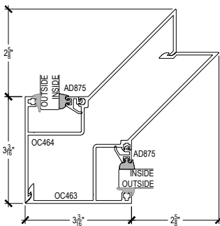
6-1 90° OUTSIDE CORNER ASSEMBLY
