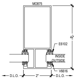
VERTICAL 4-1
