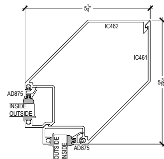
6-2 90° INSIDE CORNER ASSEMBLY
