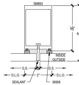
SSG VERTICAL 4-3
