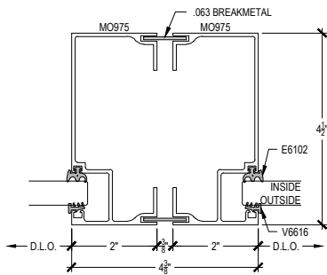
VERTICAL 4-4
