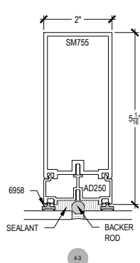
Offset Glazed
