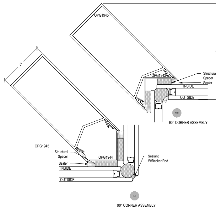
90° CORNER ASSEMBLY
