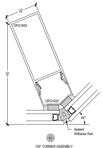
135° CORNER ASSEMBLY
