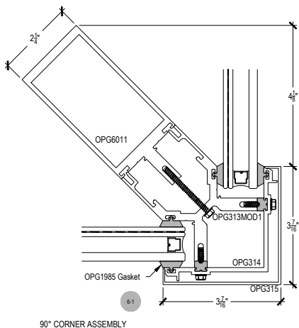
90° CORNER ASSEMBLY
