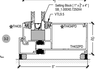
COMPENSATING STICK OUTSIDE SET
