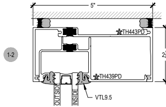
Offset Glazed
