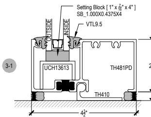
SHEAR BLOCK INSIDE SET Continuous Head / Sill
