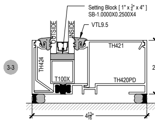
COMPENSATING STICK INSIDE SET
