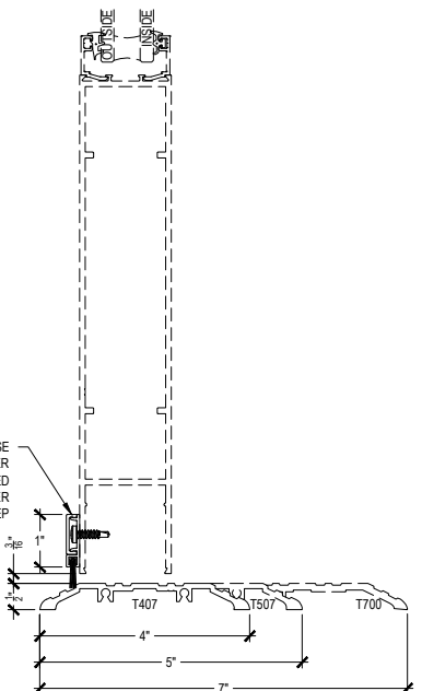
OPTIONAL THRESHOLDS @ OFFSET HUNG DOOR
