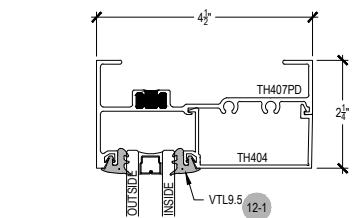
HEAD @ TRANSOM PUNCHED
